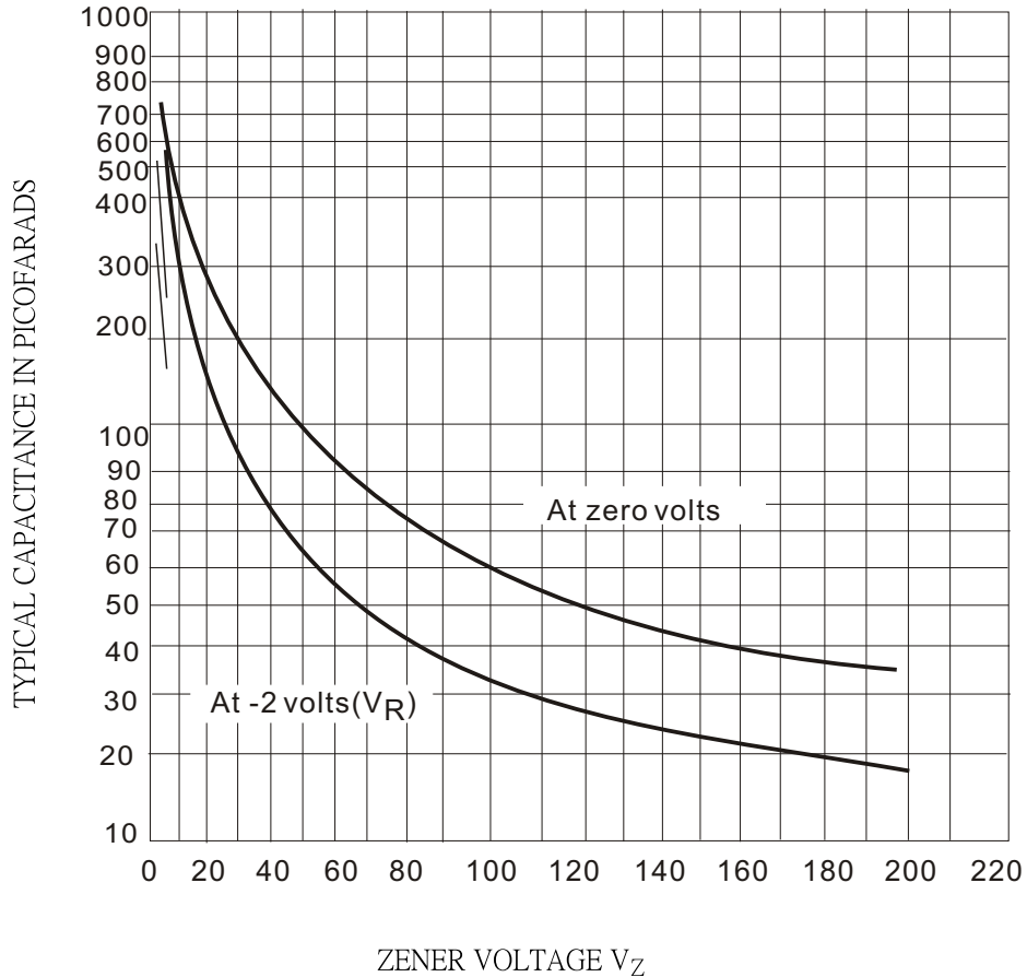
FIGURE 3 - CAPACITANCE vs. V_Z CURVE
