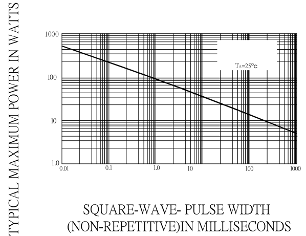
FIG.2- TRANSIENT SURGE CAPABILITY
